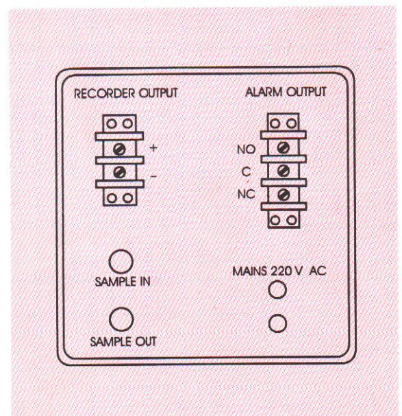
REAR VIEW
